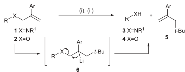
Scheme 1 Deprotection of 2-aryllallyl amines and amides 1 and ethers 2 . Reagents and conditions: (i) t -BuLi, THF, –78 to 0 °C for X = NR 1 and –78 °C for X = O; (ii) H 2 O.
